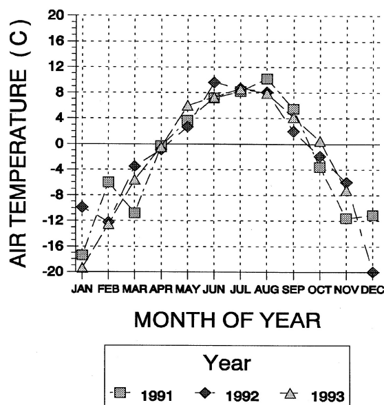
MINIMUM DAILY AIR TEMPERATURE BEAVERLODGE RESEARCH STATION
