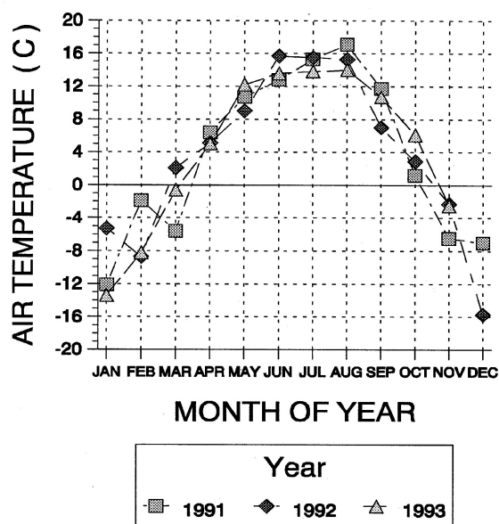
MEAN DAILY AIR TEMPERATURE BEAVERLODGE RESEARCH STATION
