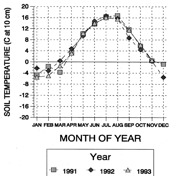
MEAN DAILY SOIL TEMPERATURE BEAVERLODGE RESEARCH STATION
